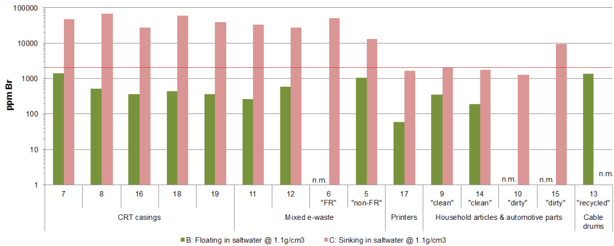
Figure 27: Bromine levels in fractions floating and sinking in saltwater with a density of 1.1g/cm 3 . In case of duplicates (6C, 7C, 11C, 12B, 17B), the average value is indicated. Samples 6B, 10B, 15B and 13C were not analysed (n.m.) due to their small size (<20g). The red line indicates the 2000ppm Br level, above which plastics must be treated in facilities capable of removing plastics with BFRs according to the CENELEC standard (CENELEC, 2014).
